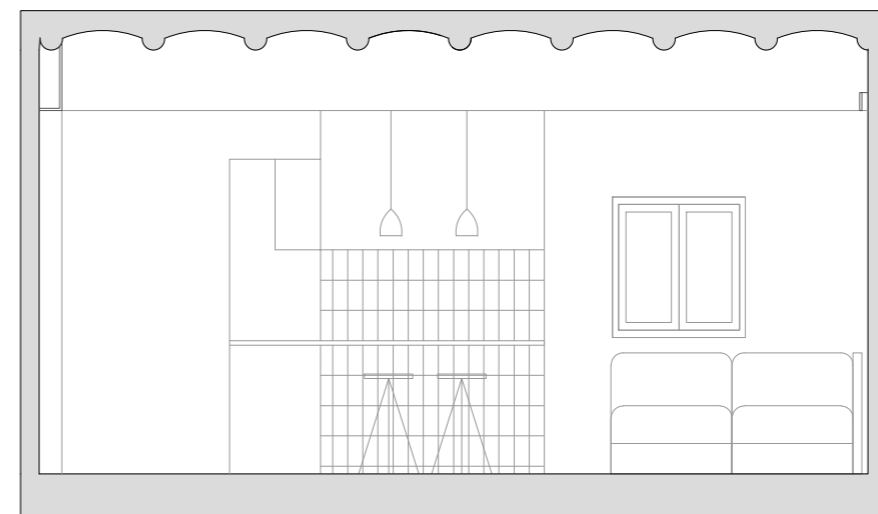
Sant Bertran_Transversal Elevation Living E:1/50
