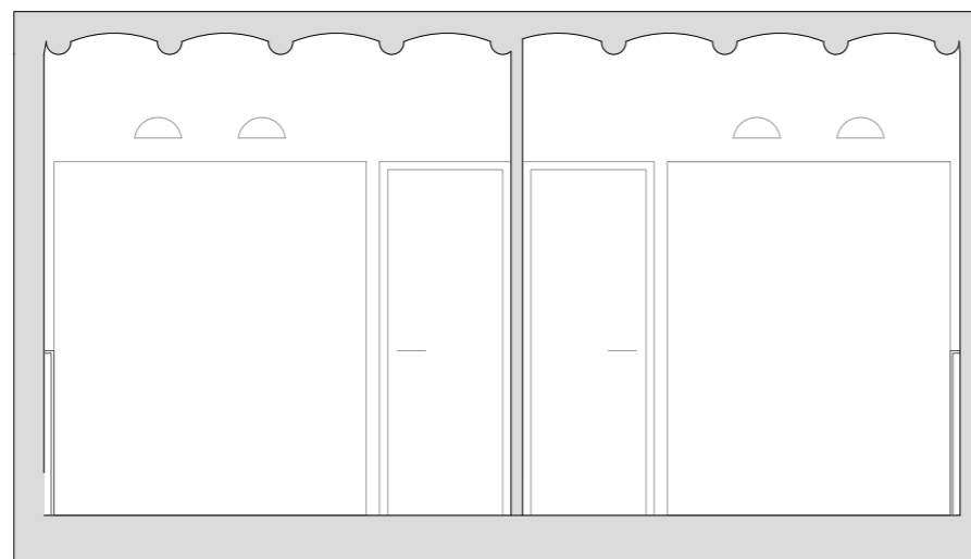
Sant Bertran_Transversal Elevation Bedrooms E:1/50
